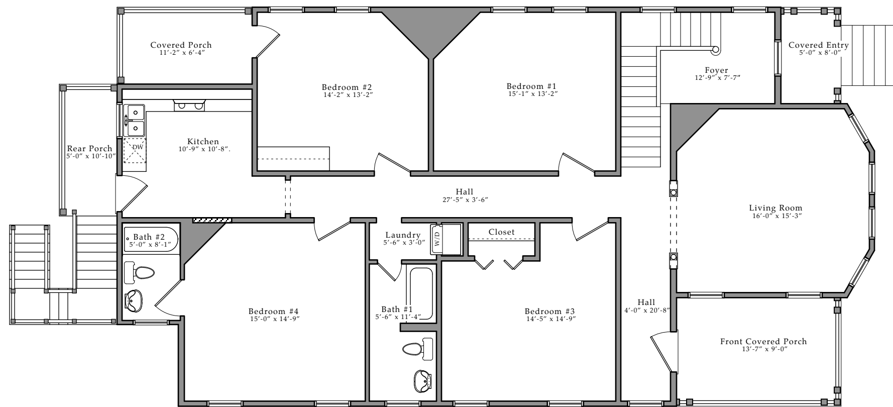
1 A1.1 UNIT "B" FLOOR PLAN
